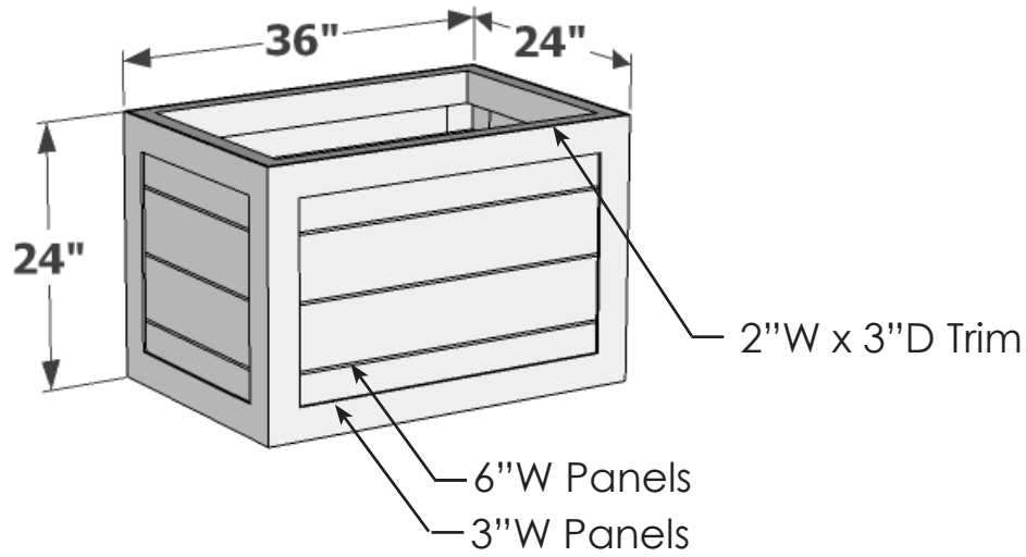
PERSPECTIVE VIEW
