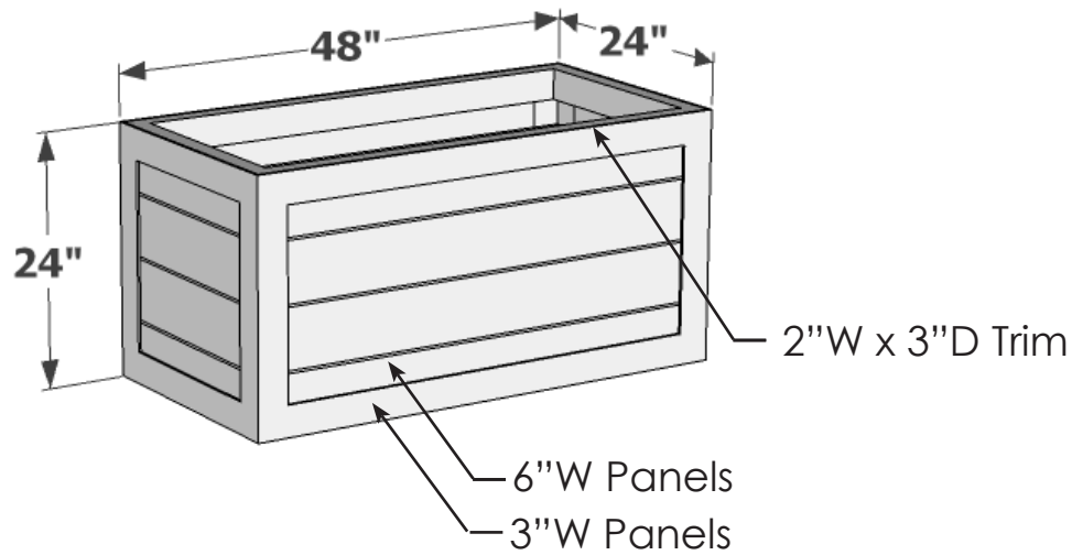
PERSPECTIVE VIEW
