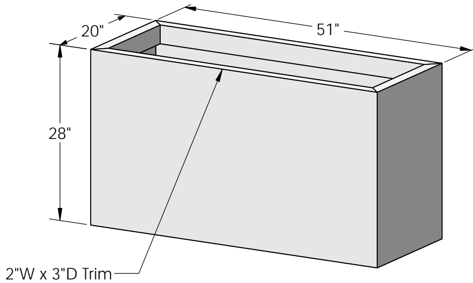
PERSPECTIVE VIEW
