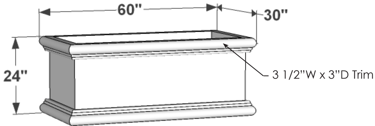
PERSPECTIVE VIEW
