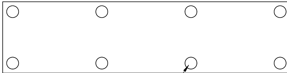
(8) Pads, 3" Dia. x 1/4" thk. Offset 1" from edges
