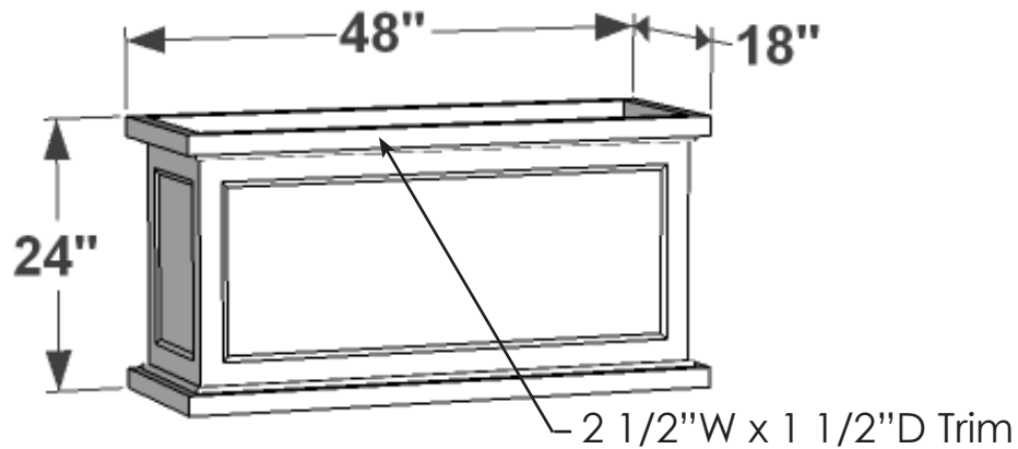
PERSPECTIVE VIEW
