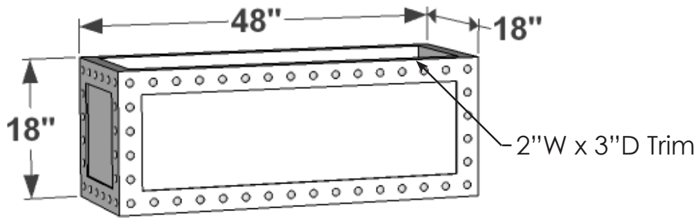
PERSPECTIVE VIEW
