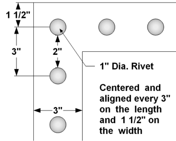
TRIM DETAIL
