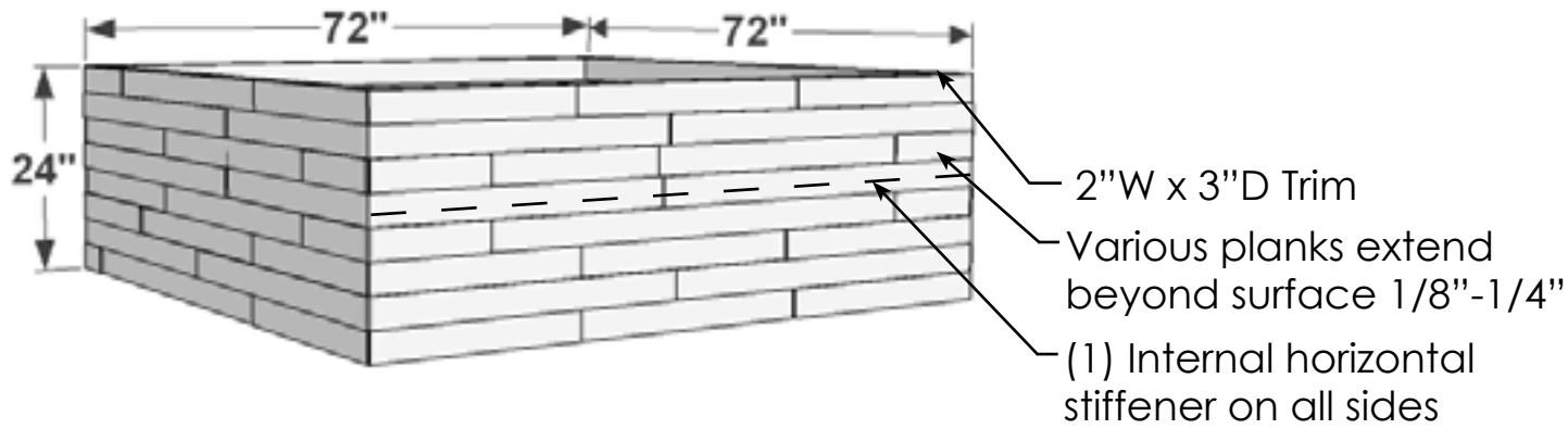
PERSPECTIVE VIEW
