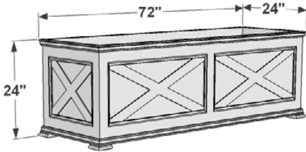
PERSPECTIVE VIEW
