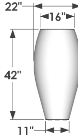
ELEVATION VIEW
