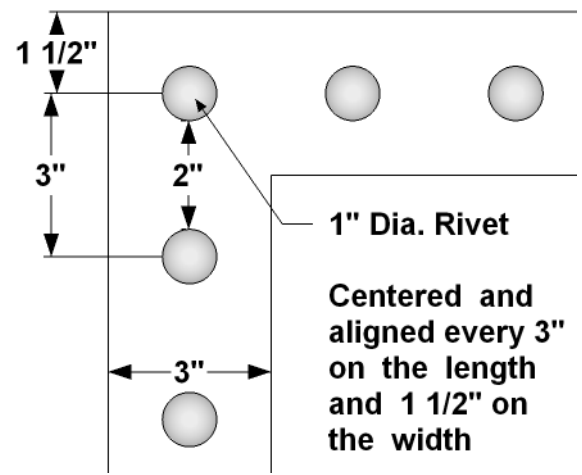
TRIM DETAIL VIEW
