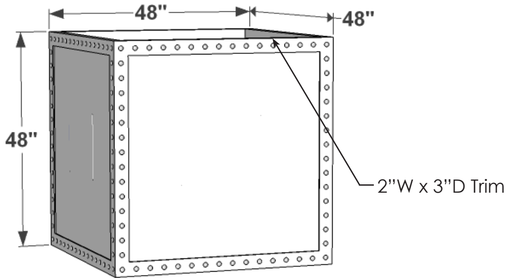
PERSPECTIVE VIEW
