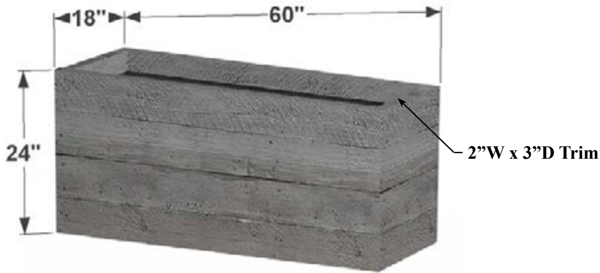
PERSPECTIVE VIEW
